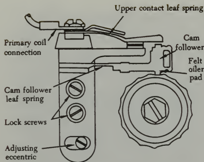
FIGURE 4-7. Pivotless type breaker assembly and cam.
